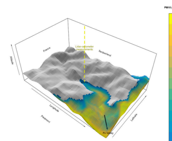
Figure 9. 3-D simulation of PM 10 concentration by FARM (image from 28 August 2015 at 15:00 UTC). The image clearly shows the entrance of the aerosol-rich air mass from the Po basin into the Aosta Valley (yellow-blue area).
