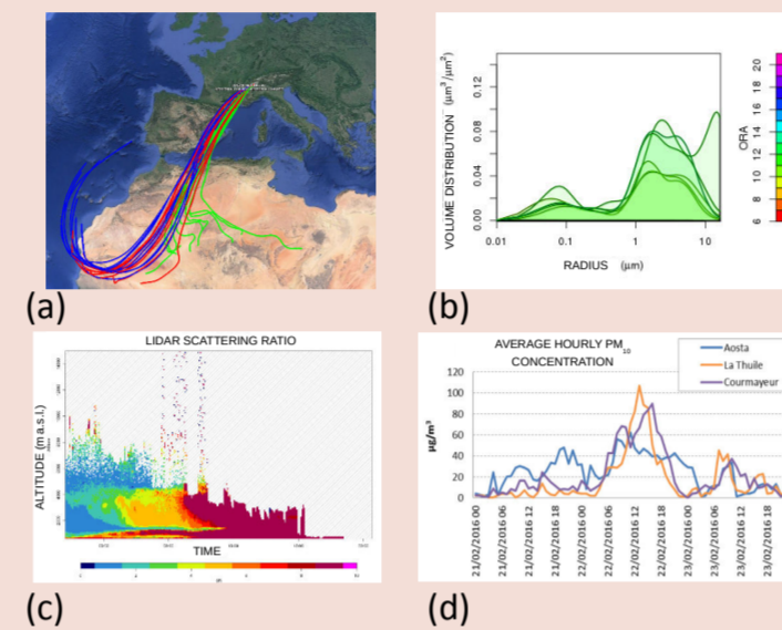
Figure 5. Backtrajectories (a), particle size distribution from the sun photometer (b), scattering ratio from the ALC (c) and surface PM 10 concentration at multiple stations (d) on February, 22 nd 2016.
