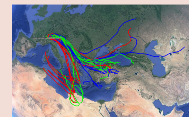
Figure 8. Transport of mineral dust from the Caspian lowlands, March, 28 th 2020.
