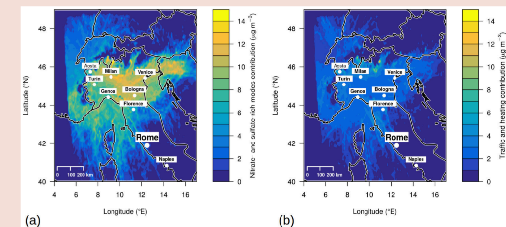
Figure 6. Concentration field trajectory statistical model using the results of the chemical analyses on aerosol samples for particles originating from secondary processes (a) and combustion (b).
